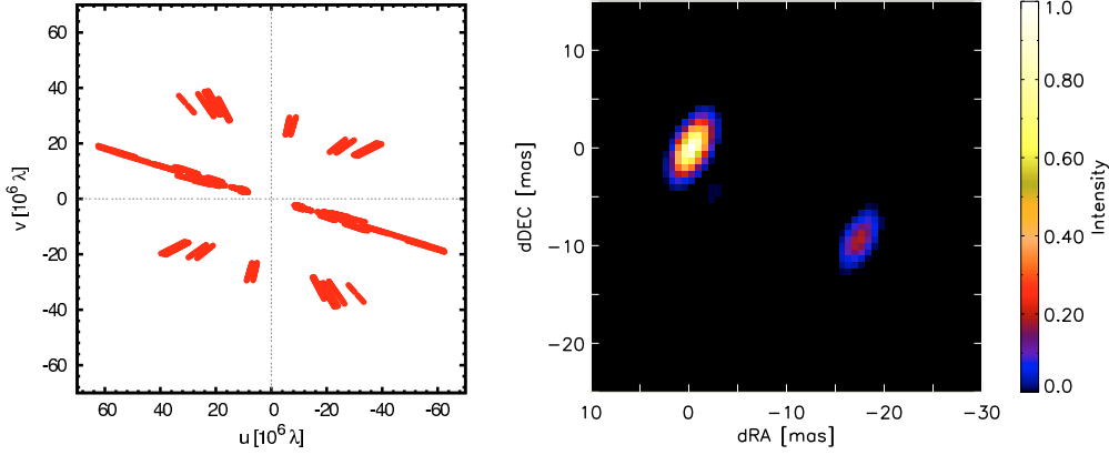
Fig. 7. Combining AMBER data obtained on three telescope configurations ( left: uv-coverage ), we reconstructed an aperture synthesis image of the \theta^1 Ori C system with an effective resolution of \sim 2 mas ( right ). For a detailed description, we refer to Sect. 4.
