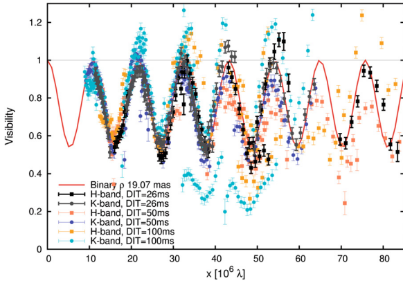
Fig. 4. AMBER visibilities measured on 2007 Dec. 03 and 2007 Dec. 05 plotted versus projected distance in the uv -plane (where the projection was perpendicular to the fitted binary separation vector \Theta = 241.2^\circ , i.e. x = u \cos(\Theta + 90^\circ) - v \sin(\Theta + 90^\circ) ). The solid red line shows the theoretical cosine visibility profile for a binary star with separation 19.07 mas and intensity ratio 0.30. As indicated by the strong visibility offsets, which particularly occur at high spatial frequencies, the absolute calibration is sometimes rather poor, reflecting the changing atmospheric conditions during these nights. It can also be seen that this calibration bias is particularly important for long DITs (50 ms, 100 ms), while it is nearly negligible for short DITs (26 ms, grey & black points). As expected, the spectral dependence of the visibility is not affected by these calibration uncertainties.
