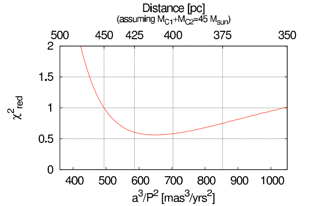
Fig. 12. Minimum \chi_r^2 curve as a function of a^3/P^2 = (M_{\text{system}}) \cdot \pi^3 , through which the dynamical orbital parameters can be related to the mass sum and the dynamical parallax. For illustration, we give the dynamical distance in the upper axis assuming a total system mass of 45 M_{\odot} .
