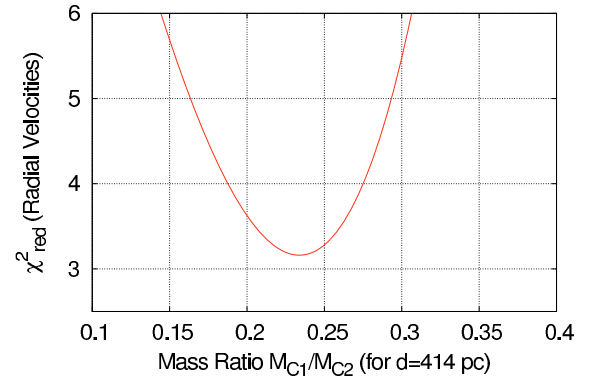
Fig. 11. \chi_r^2 curve for our fit of the binary mass ratio to the available radial velocity data (assuming a distance of 414 pc). We assume the orbital elements (Table 4) derived from our interferometric measurements.
