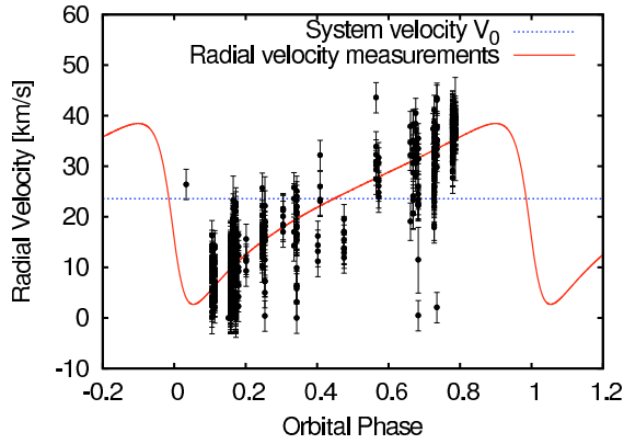
Fig. 10. The radial velocities measured towards \theta^1 Ori C plotted as function of orbital phase (assuming the orbital elements determined with our grid search algorithm; see Table 4). Besides the extensive data set by Stahl et al. (2008) , we included the radial velocities measured by Struve & Titus (1944) , Conti (1972) , and Morrell & Levato (1991) . The red line shows the radial velocities corresponding to our orbital solution with a system velocity V_0 = 23.6 \text{ km s}^{-1} (blue dashed line) and the mass ratio q(414 \text{ pc}) = 0.23 as determined from our least-square fit (Sect. 5.2).
