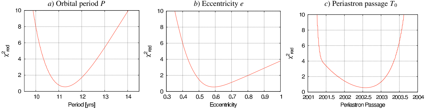
Fig. 9. Minimum \chi_r^2 curves as function of the dynamical orbital parameters P , e , T_0 . These curves were used to determine the best-fit orbit solution and to evaluate the uncertainties on the individual parameters (see Table 4).
